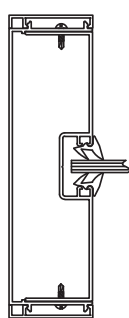
Sidelight Mullion
