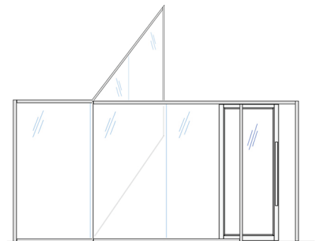
Office front with 3-way post
